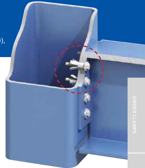
Hollo-Bolt HCF (High Clamping Force) See page 51
